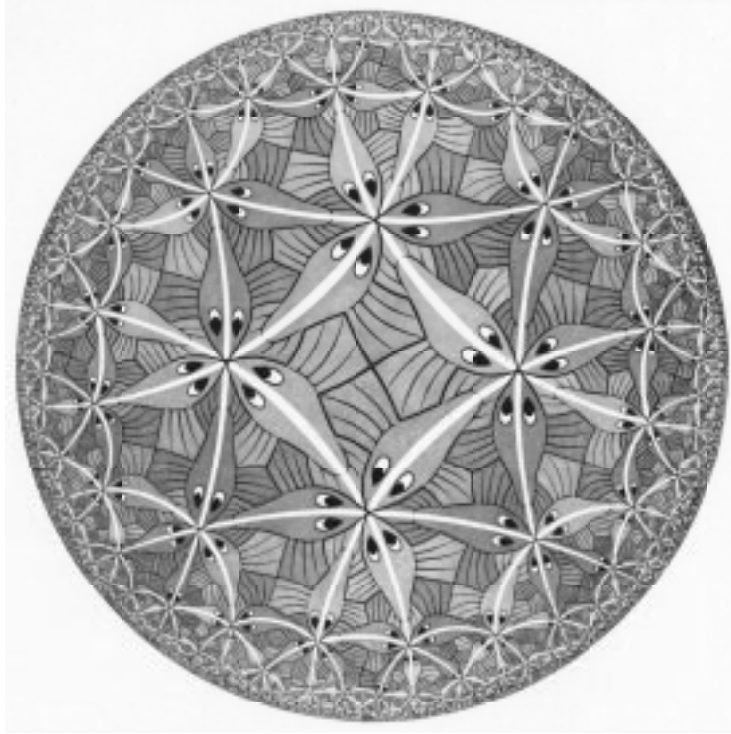
FIGURE 3.9.5 M. C. Escher's "Circle Limit III". Every fish is the image of every other by an isometry of \mathbf{D} . © the M. C. Escher Company-Holland. All rights reserved. www.mcescher.com .
